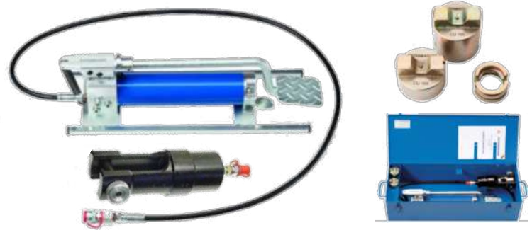
Hydraulic Crimping Tool Set with Foot Pump in blue metal case
